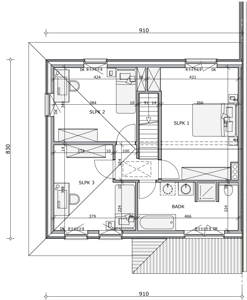
VERDIEPING Opp.= 75.36 m 2
